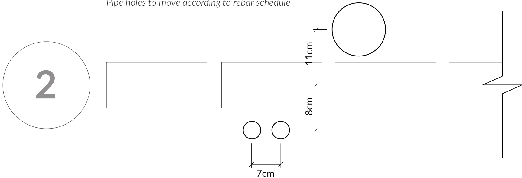
2 Plan 1:5 Plumbing Hole Detail
